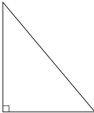
Right Triangle
