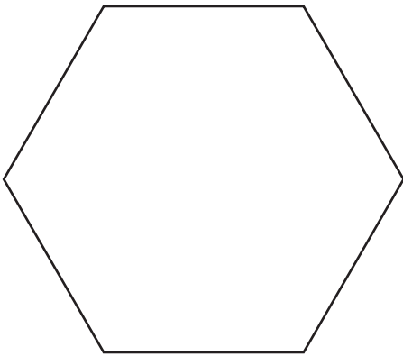
Regular Hexagon
