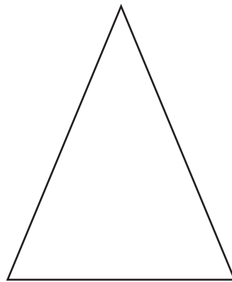
Isosceles Triangle
