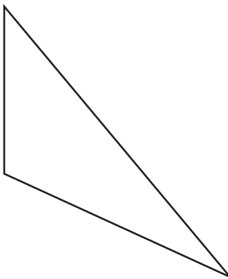
Obtuse Triangle
