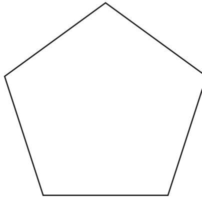
Regular Pentagon
