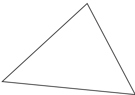
Scalene Triangle
