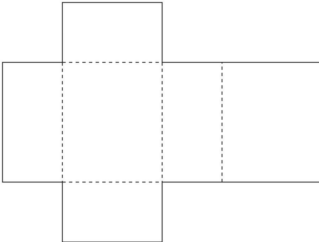
Rectangular Prism
