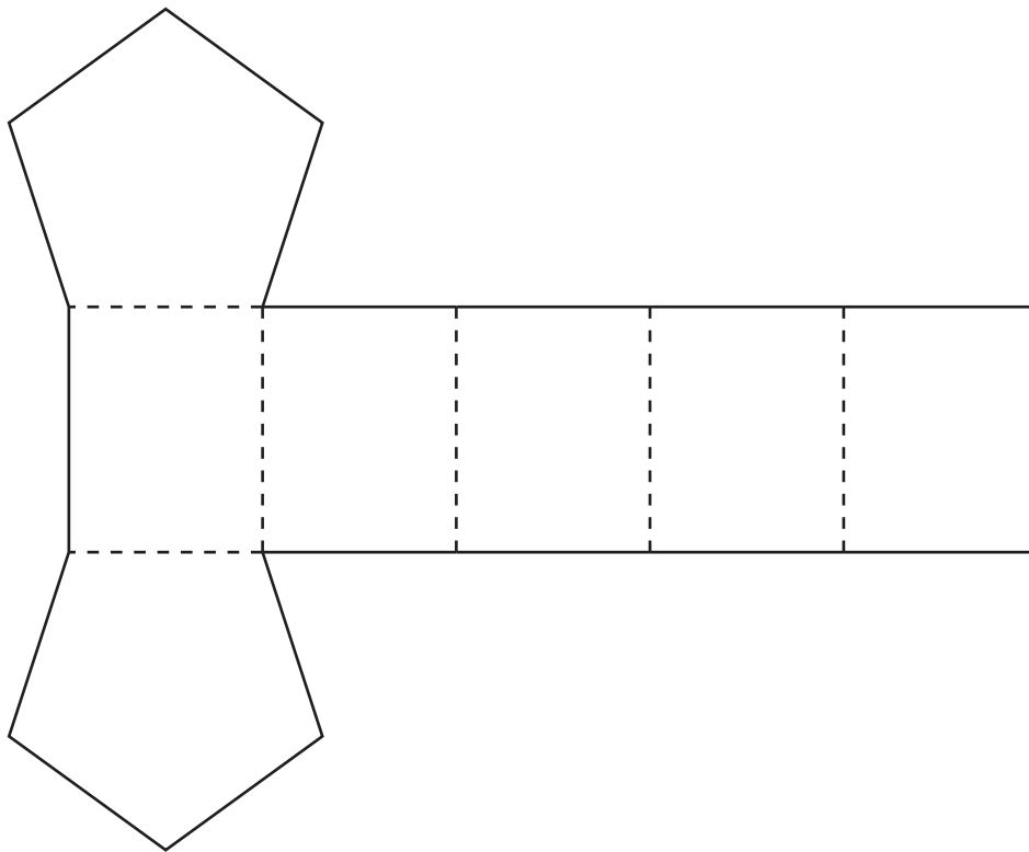
Pentagonal Prism
