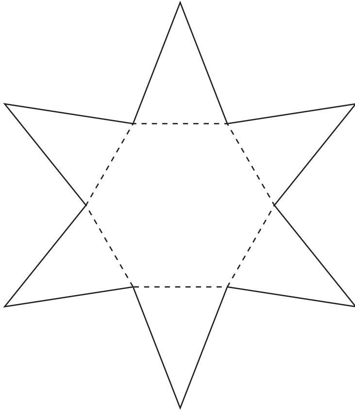
Hexagonal Pyramid
