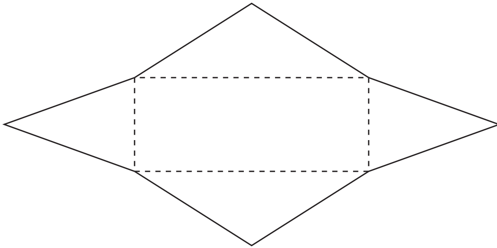
Rectangular Pyramid
