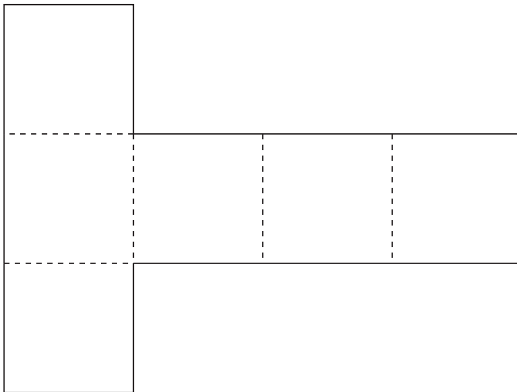
Cube
