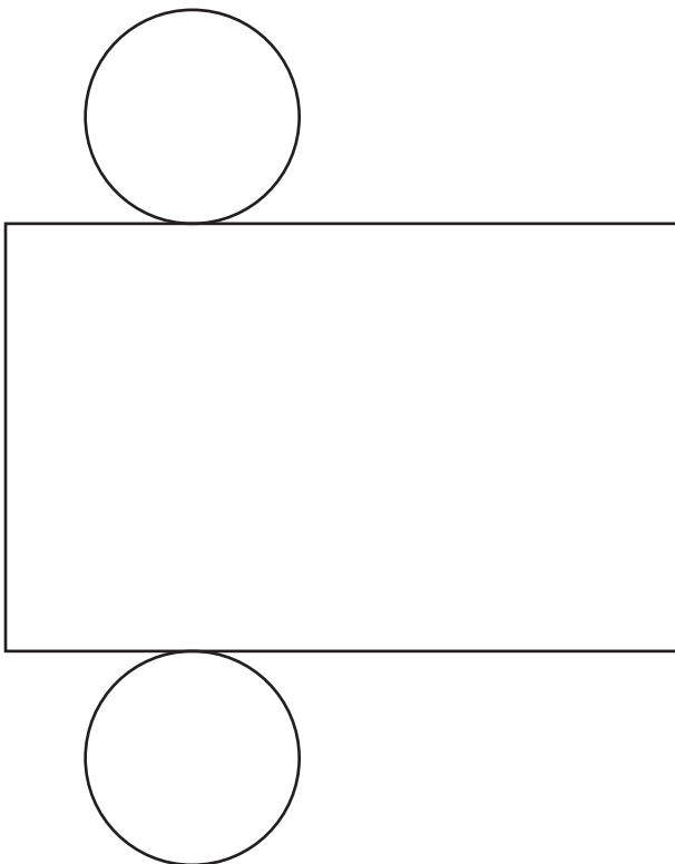
Cylinder
