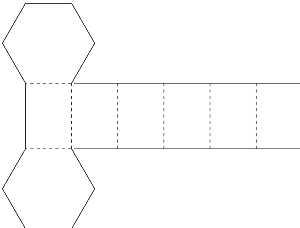
Hexagonal Prism
