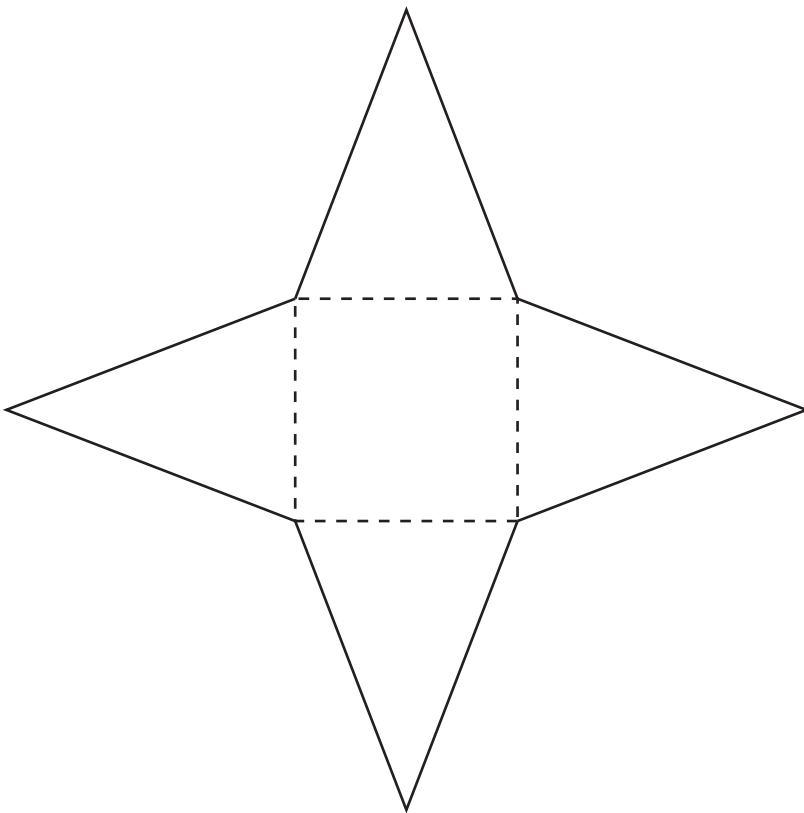
Square Pyramid
