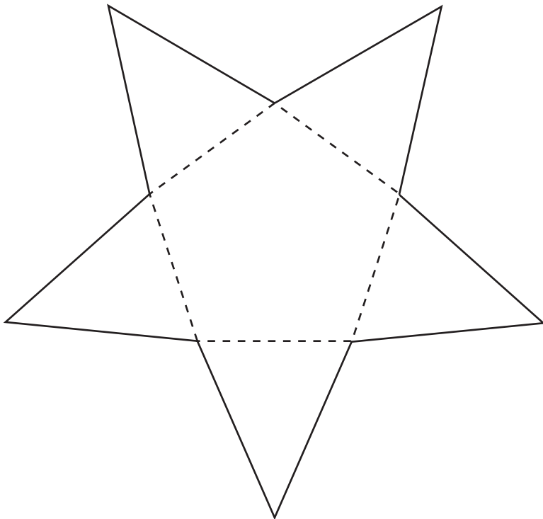
Pentagonal Pyramid
