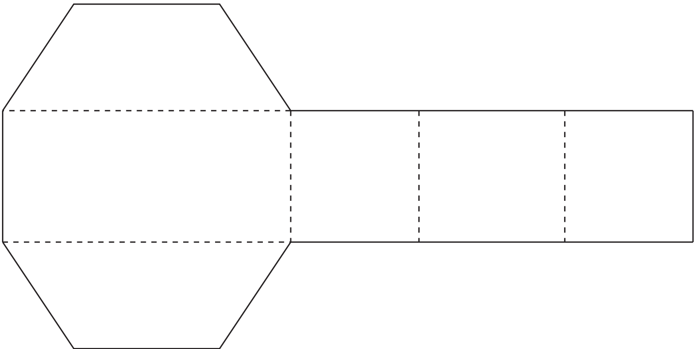
Trapezoidal Prism
