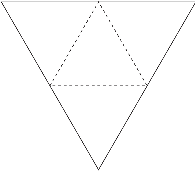
Tetrahedron
